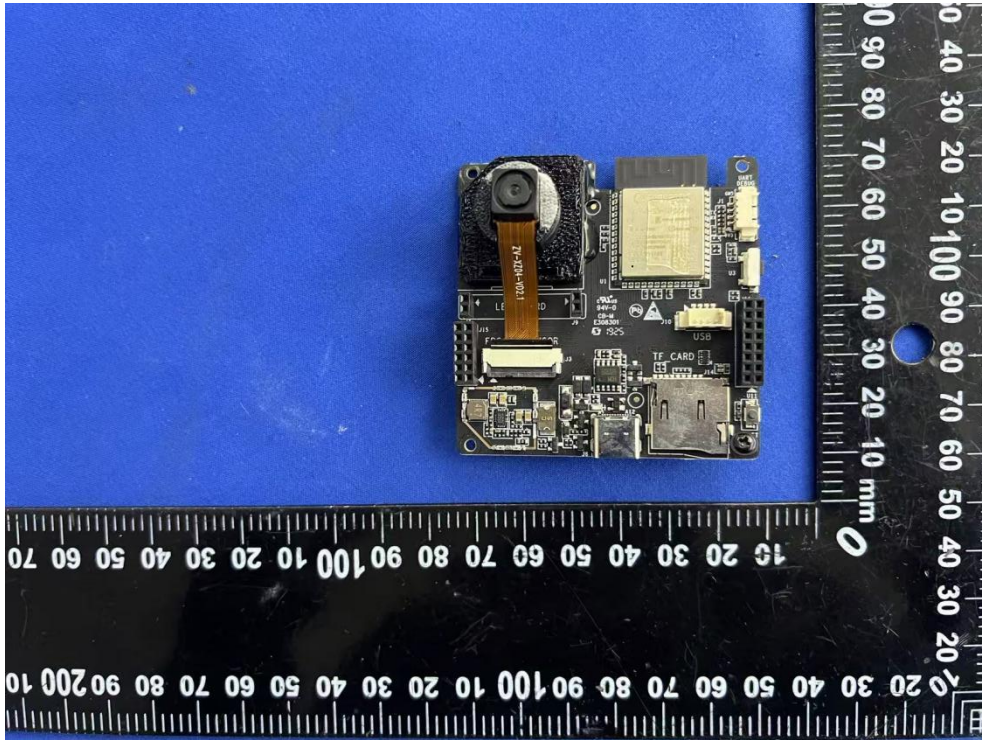
Picture 5 NE100-MB01 board
