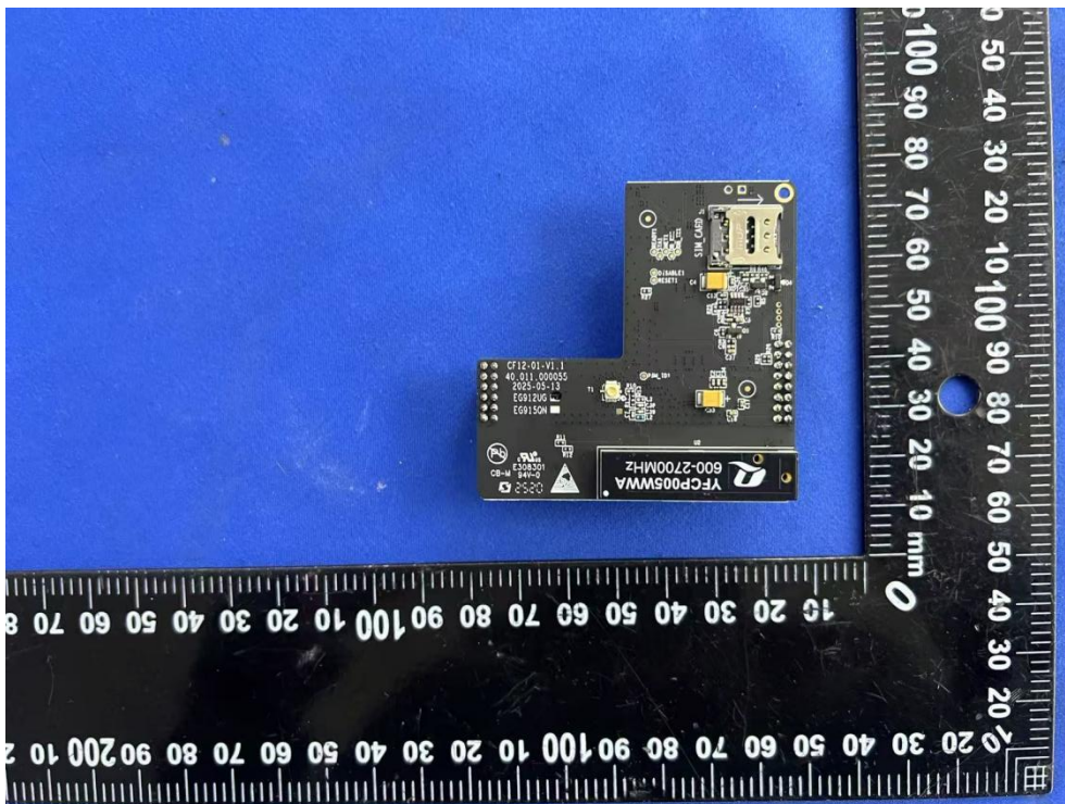
Picture 4 NeoEyes NE-CM01 Cat-1 Module board
