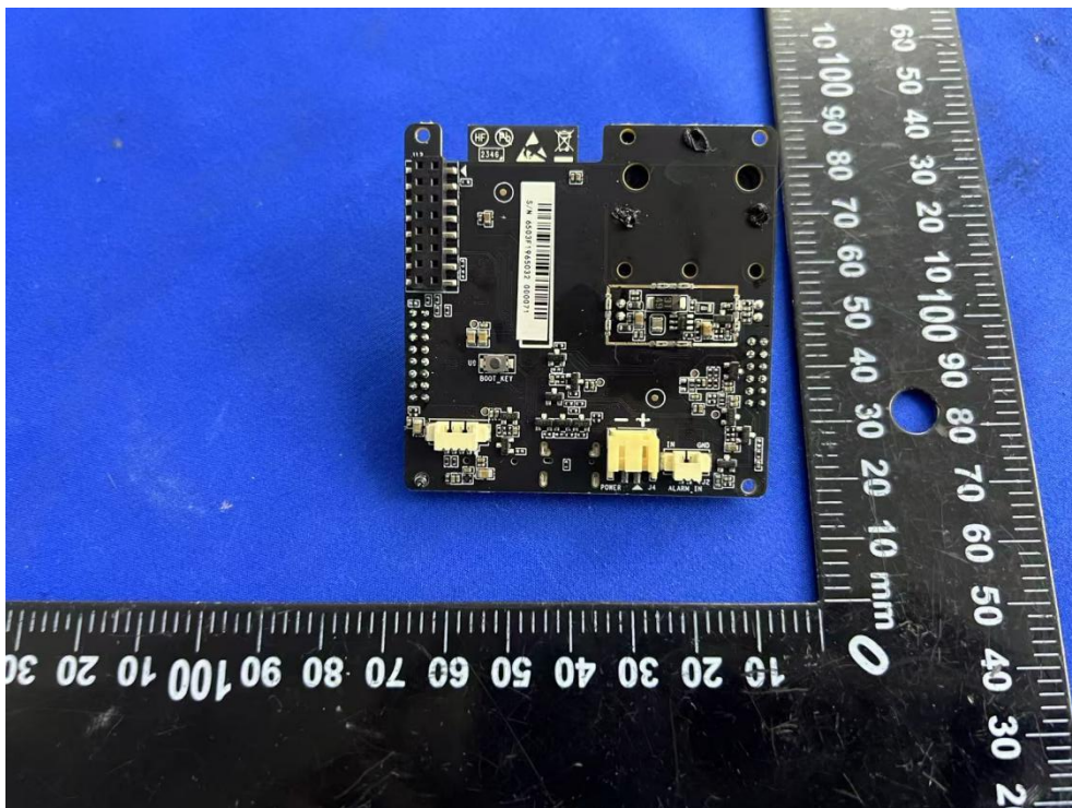
Picture 6 NE100-MB01 board
