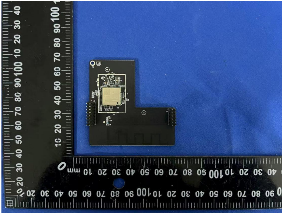
Picture 3 NeoEyes NE-CM02 WiFi-HaLow Module board
