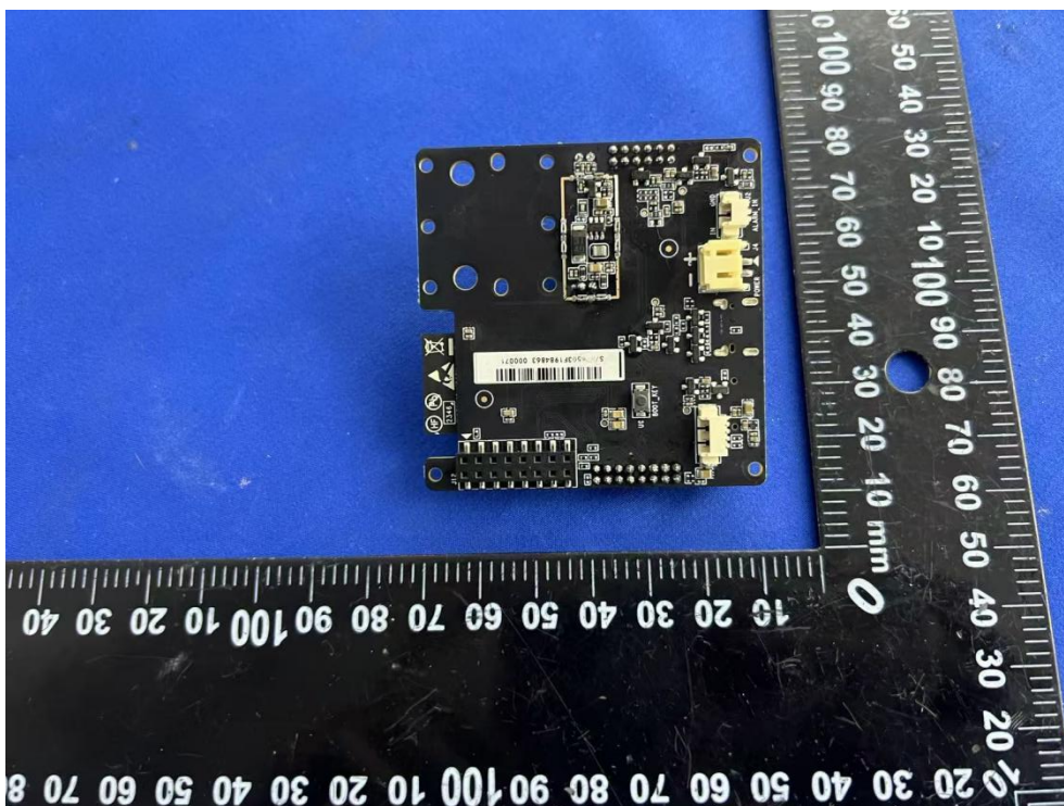
Picture 2 NeoEyes NE100-MB01 Development Board
