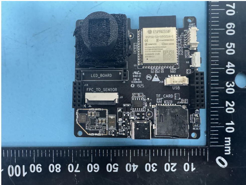
Picture 7 NE100-MB01 board
