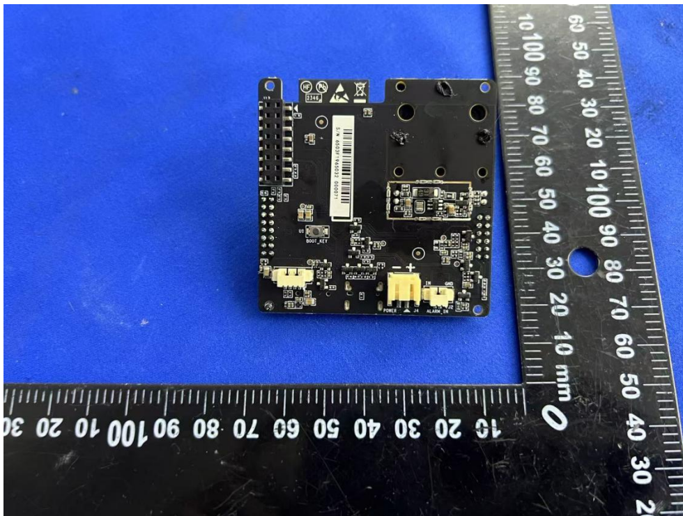
Picture 8 NE100-MB01 board
