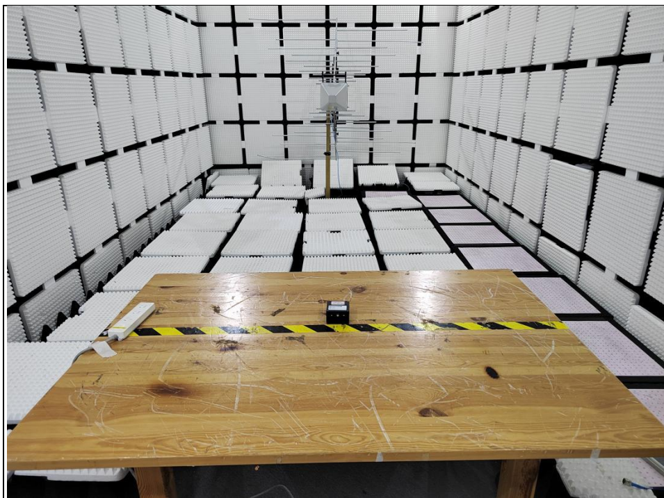
RS TEST
