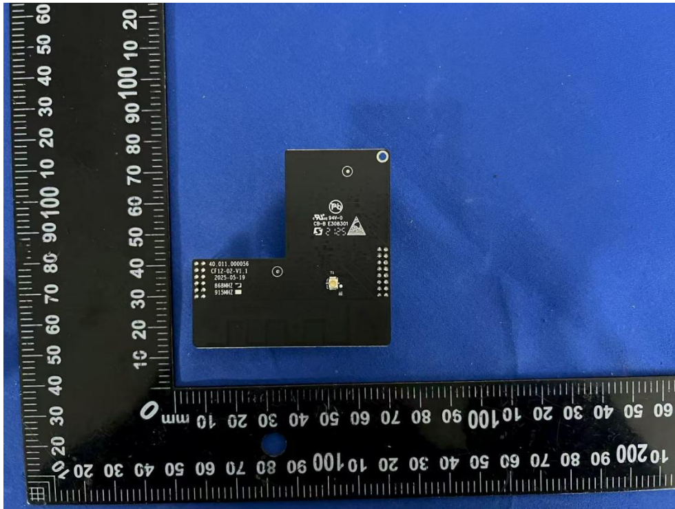
Picture 9 NeoEyes NE-CM02 WiFi-HaLow Module board
