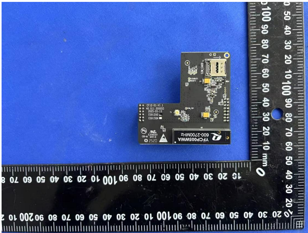
Picture 9 NeoEyes NE-CM01 Cat-1 Module board
