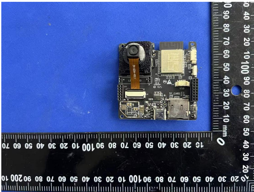
Picture 10 NE100-MB01 board
